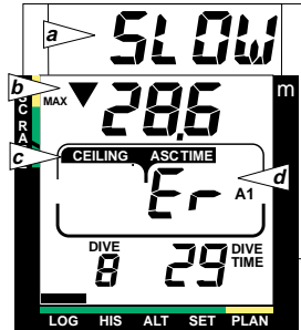
Fig 4.5 VIOLATION DISPLAYS IN THE LOGBOOK, DISPLAY I
