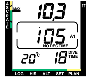
Fig. 3.12 ASCENT RATE INDICATOR Pointer at position three: ascent rate 9 - 11 m/min [30 - 36 ft/min].
