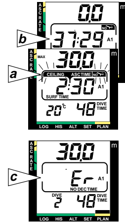
Fig. 3.18 DISPLAYS AFTER VIOLATED DECOMPRESSION DIVE
