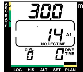
Fig. 3.6 DIVE PLANNING The no-decompression time limit at 30.0 m [100 ft] is 14 minutes in A1 mode.
