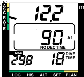
Fig. 3.11 ASCENT RATE INDICATOR
