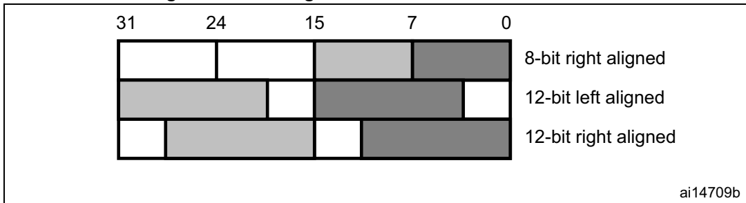
Figure 66. Data registers in dual DAC channel mode
