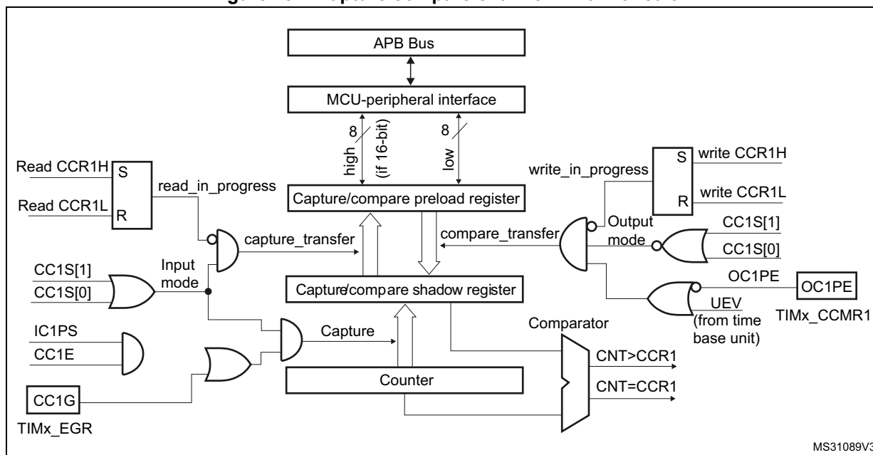
Figure 194. Capture/compare channel 1 main circuit
