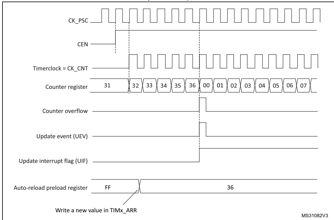
Figure 189. Counter timing diagram, update event when ARPE=1 (TIMx_ARR preloaded)
