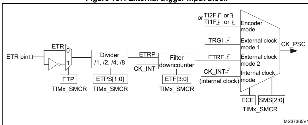
Figure 157. External trigger input block
